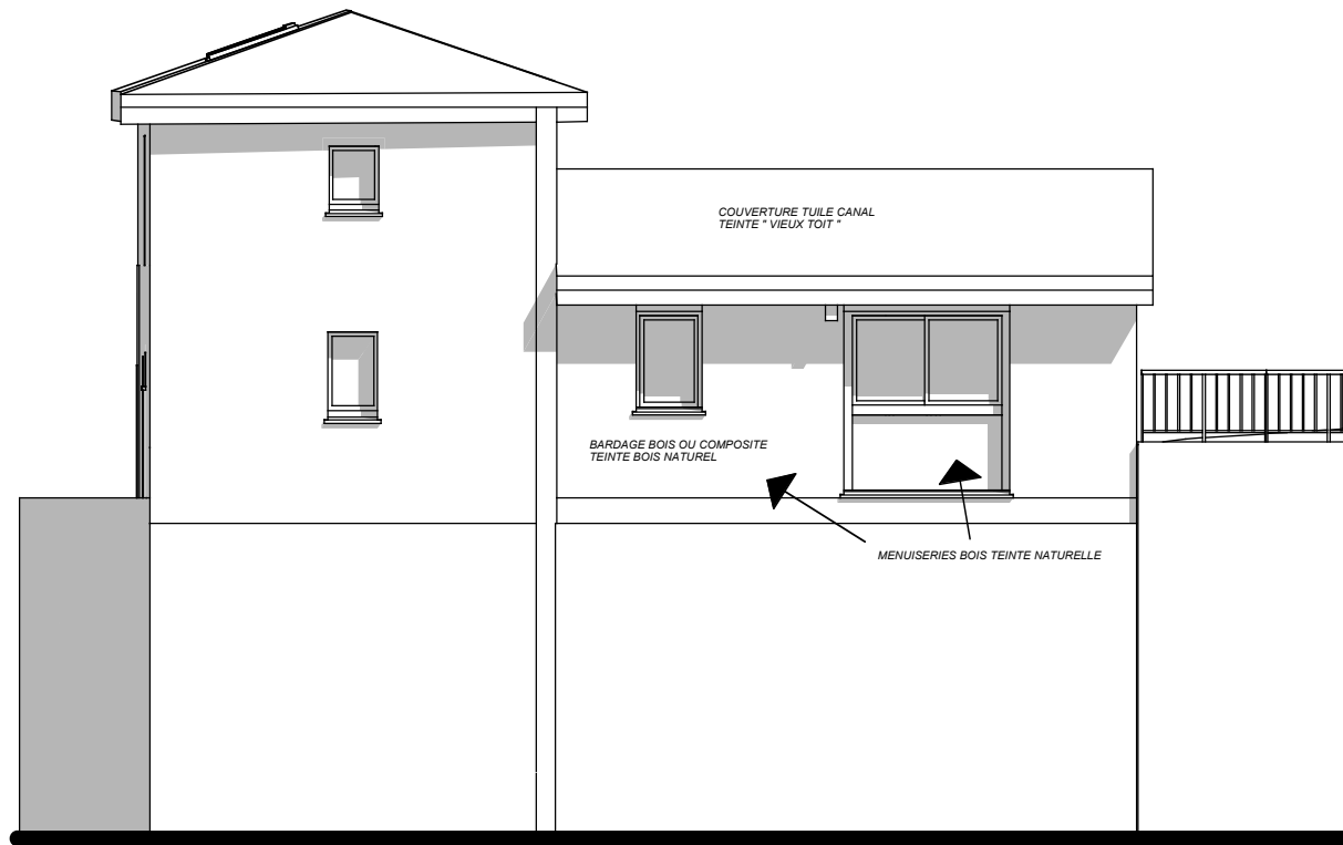
FACADE SUD
